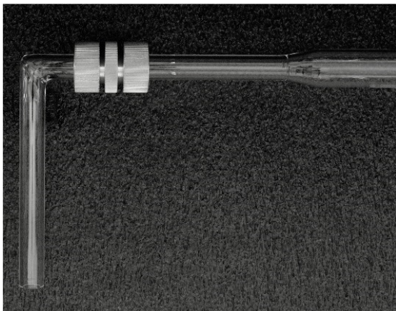
Close Up – Plasma Tube Top Section – No Ball Cup Design
