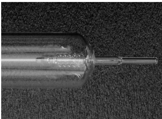
Close Up – Plasma Tube Bottom – Fused Bubbler and no Ball Cup Design
